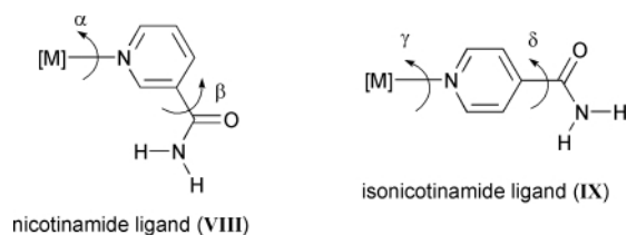
Scheme 3 Nicotinamide (pyridine-3-carboxamide) and isonicotinamide (pyridine-4-carboxamide) ligands. Curved arrows indicate torsional flexibility at positions \alpha – \delta .
