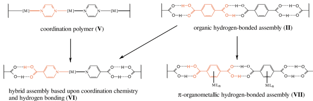
Scheme 2 Illustration of the incorporation of metals into 1D hydrogen bonded-assemblies, via coordination chemistry ( VI ) or \pi -organometallic chemistry ( VII ), and their relationship to the parent organic hydrogen-bonded assemblies ( II ) and coordination polymers ( V ).
