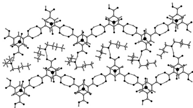
Fig. 12 Structure of 10 \cdot \text{Bu}^n_2\text{O} depicting the hydrogen-bonded zigzag ribbons of 10 and the solvent channels in which \text{Bu}^n_2\text{O} solvent molecules are anchored via an \text{O}-\text{H} \cdots \text{O} hydrogen bond as well as a number of \text{C}-\text{H} \cdots \text{O} hydrogen bonds (not shown); chromium and oxygen atoms are shaded.
