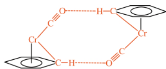
Scheme 4 R_2^2(10) hydrogen bonded linkage observed in 5 [see Fig. 8(b)].
